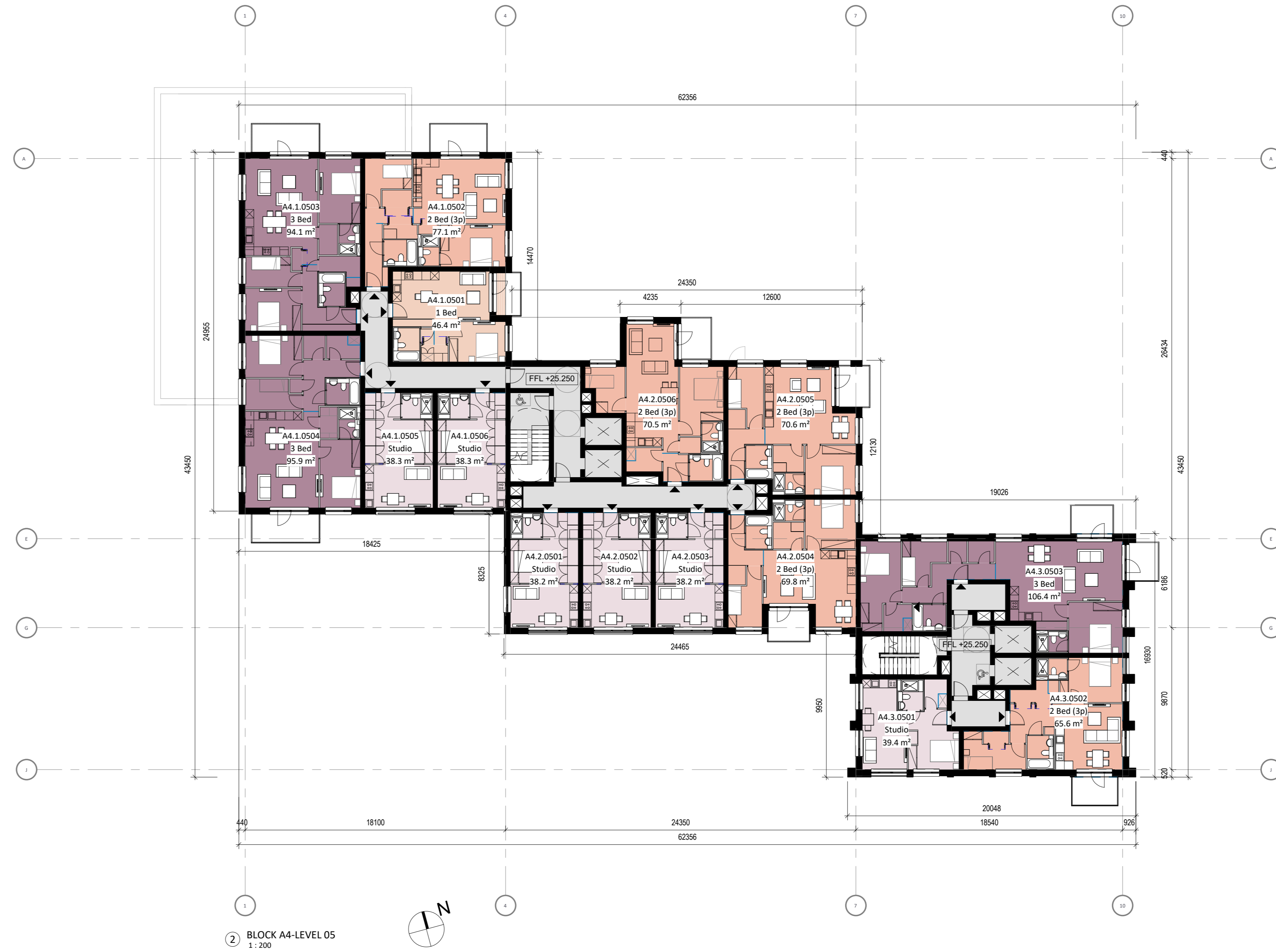
2 BLOCK A4-LEVEL 05 1:200
