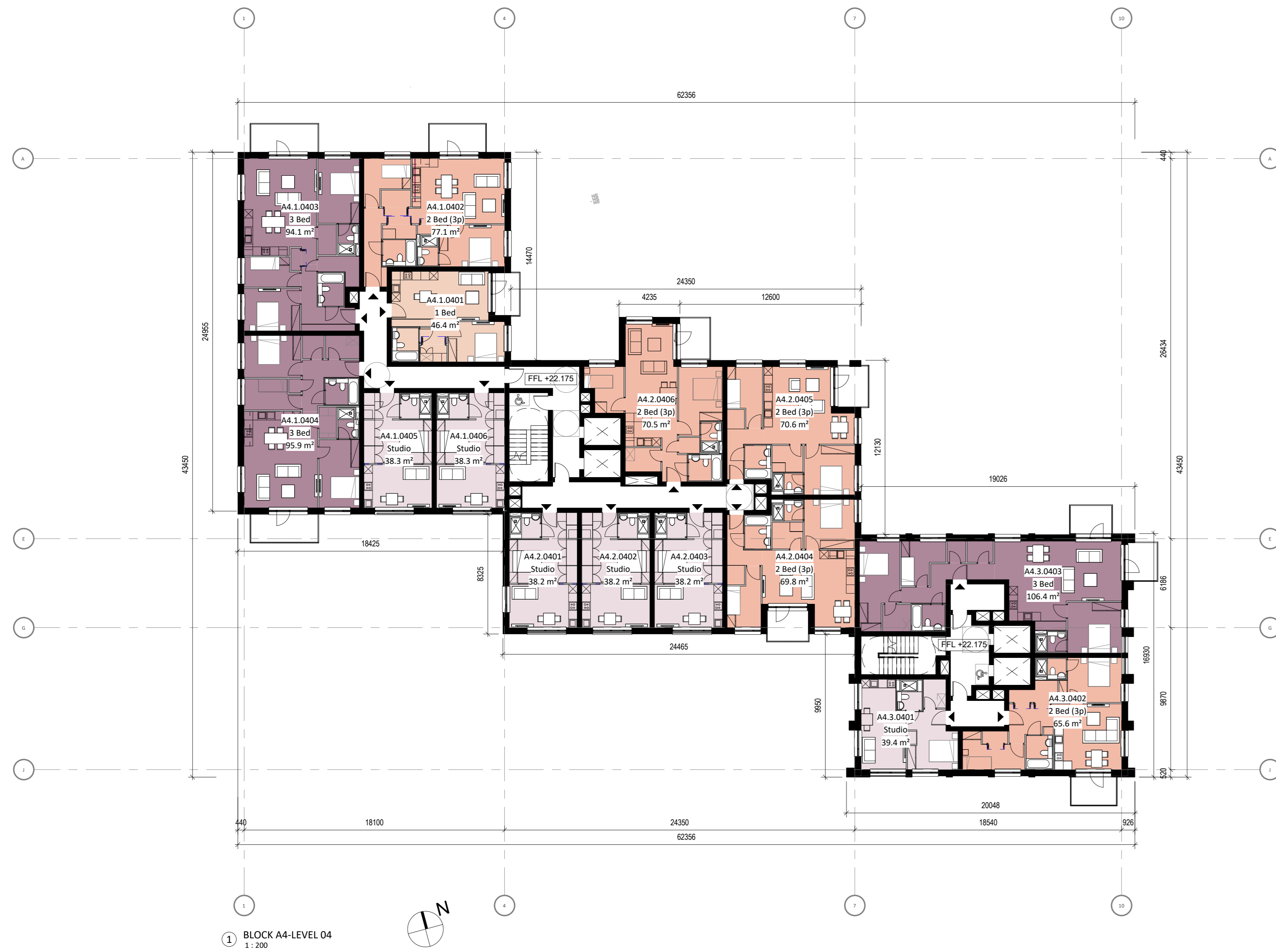
1 BLOCK A4-LEVEL 04 1:200
